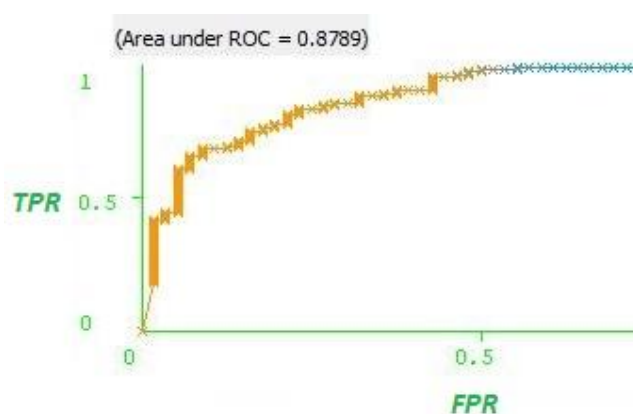
Naïve Bayes
