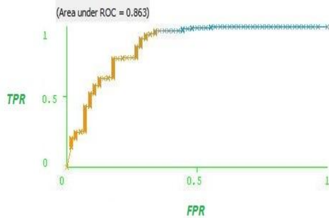
RBF
